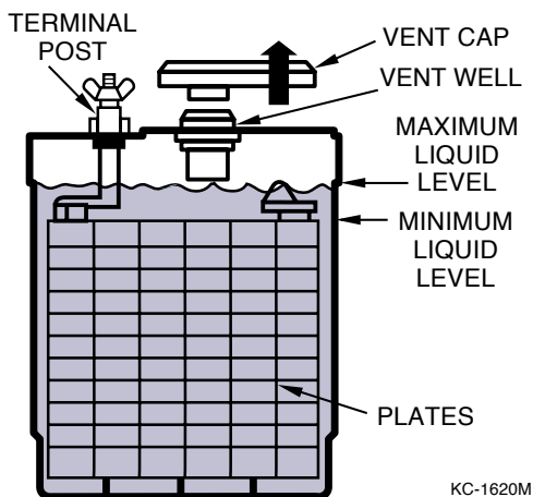
Figure 37 - Battery Level
