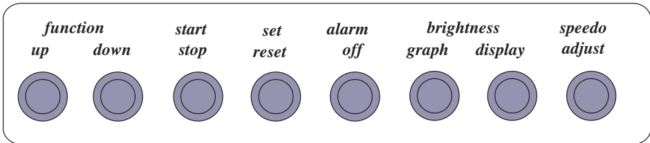
Figure 11 - Computron Control Panel
