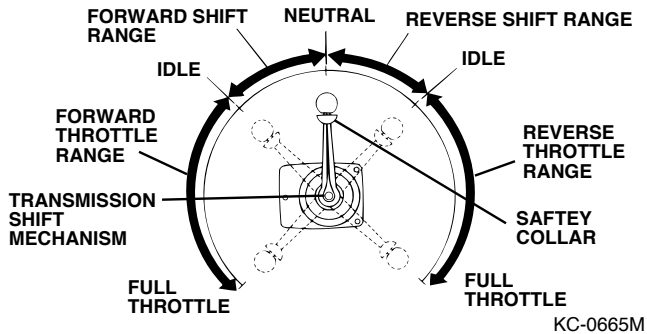
Figure 34 - Throttle Positions
