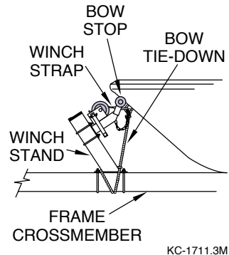
Figure 32 - Bow Tie-Down
