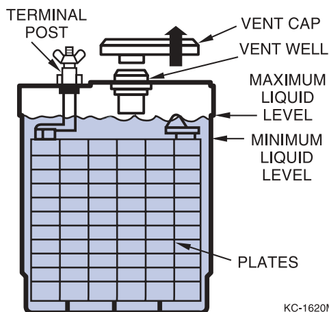
Figure 4-4. Battery Level
