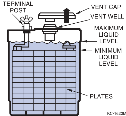
Figure 4-5. Battery Level
