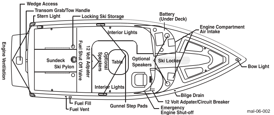
Figure 2-2. General Layout V-Drive Boats
