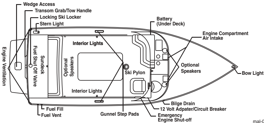
Figure 2-3. General Layout Direct Drive Boats
