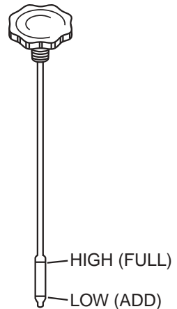
Figure 4-1. Typical Transmission Dipstick
