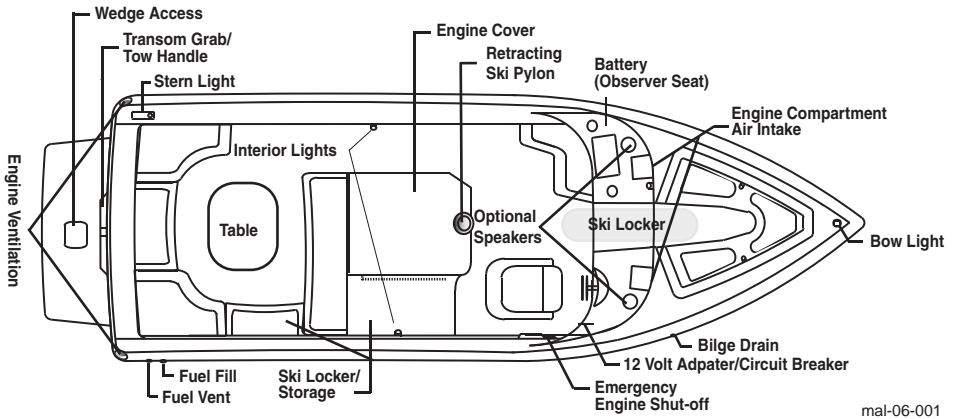
Figure 2-1. General Layout XTi Model Boats
