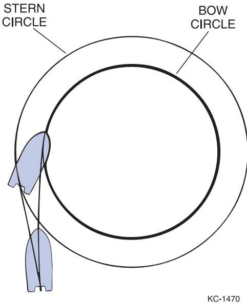
Figure 3-9. Stern Push
