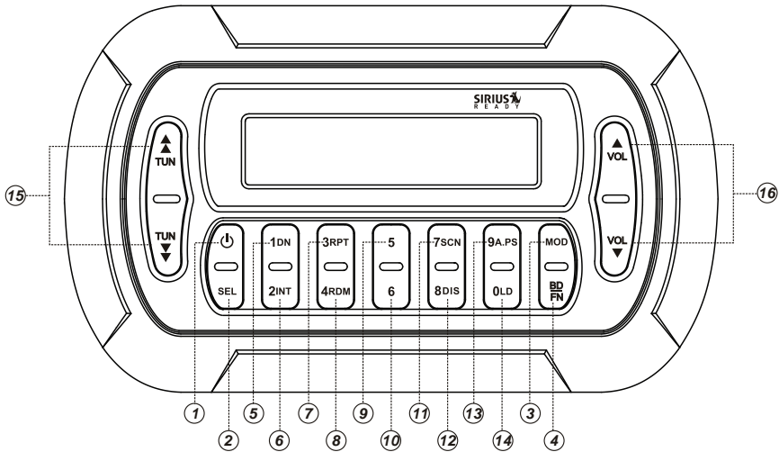
Figure 2-41. Remote Control
