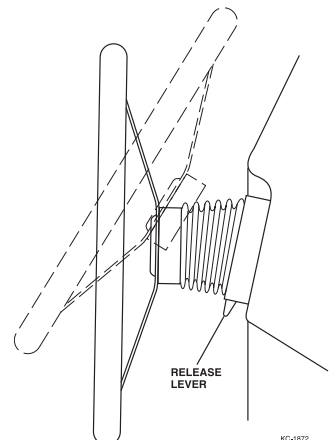
Figure 2-34. Tilt Steering
