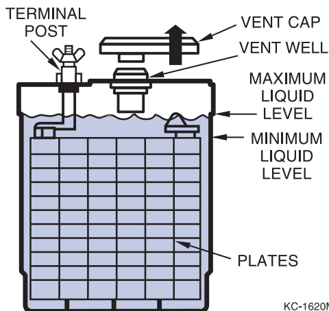
Figure 4-9. Battery Level
