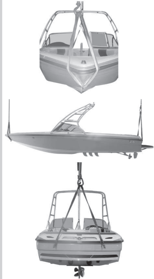
CORRECT HOISTING
